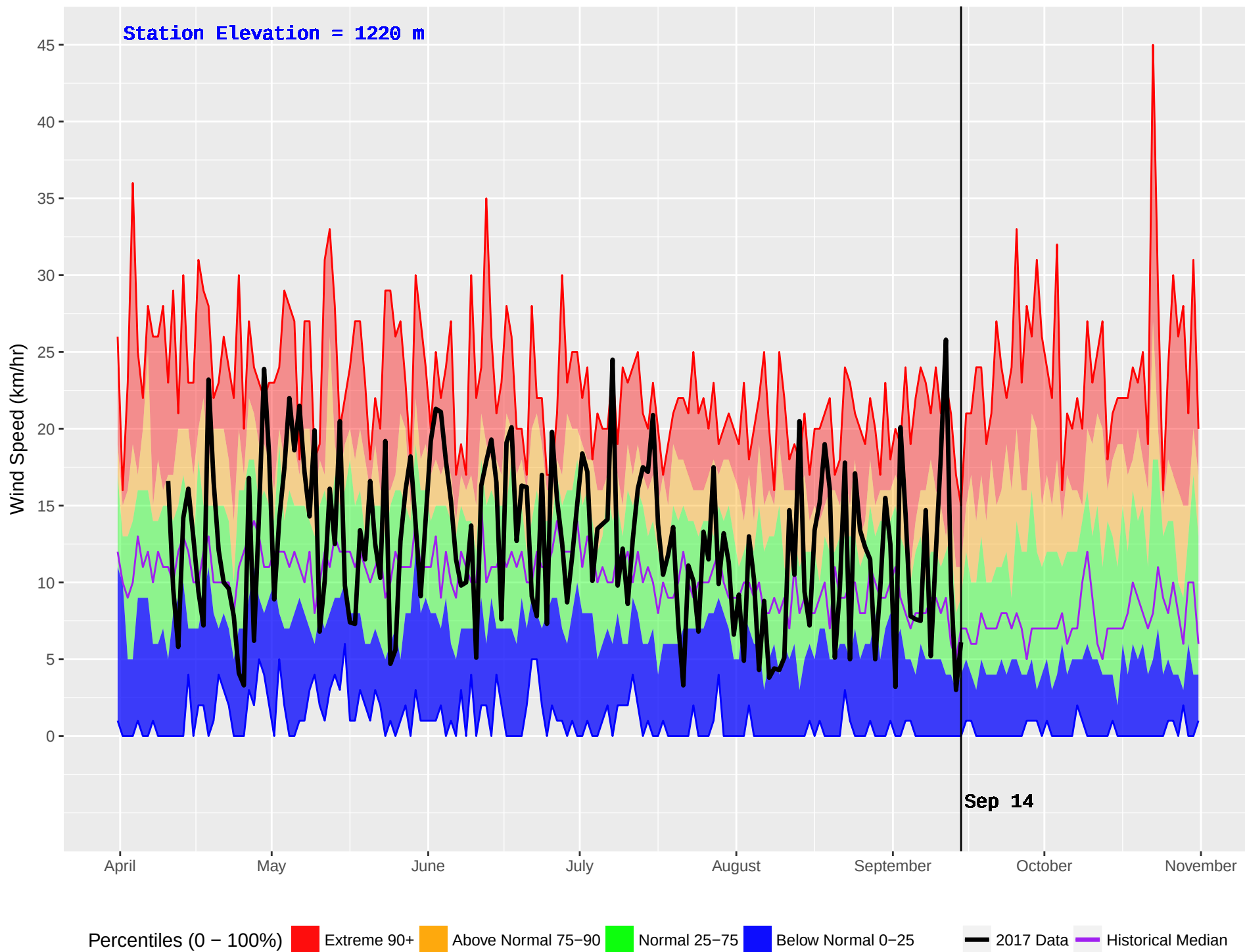
NEMIAH (216) : Historical (1982–2016) and Current (2017) Noon Wind Speed
